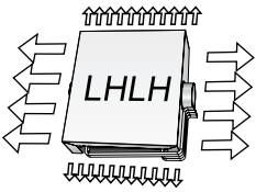
Figure 17. Nozzle setting example, ADAPT Parasol EX single-module unit - LHLH.
