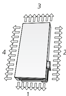
Figure 10. Top view, nozzle setting, PARASOL EX two-module unit, sides 1-4.
