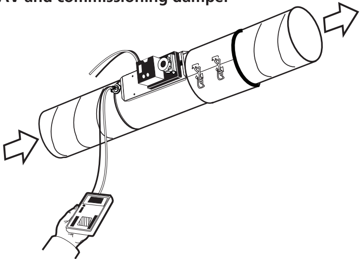
Figure 8. Example VAV/CAV. Number of measuring tubes: 2. Connected to "nipple well". The K-factor is also valid for the combination VAV with sound attenuator CLA L = 500 or 1000 mm.
