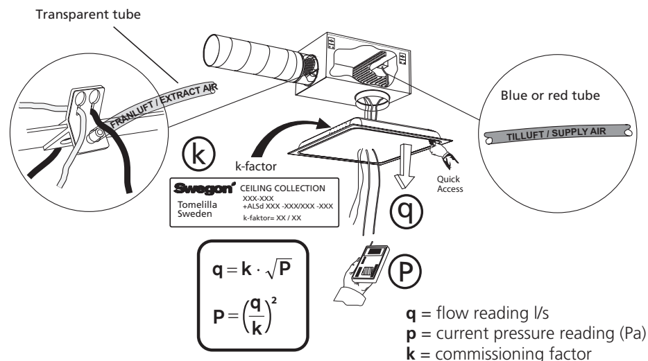
Figure 2. Example ALS, measurement with two tubes.
